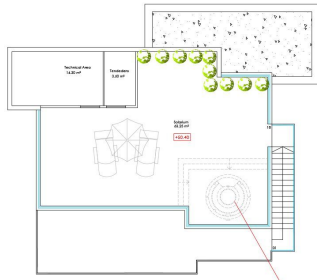
ROOF FLOOR
