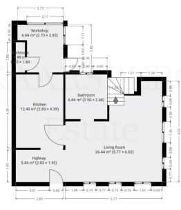
OTTO SCALE nest house - 1st floor
