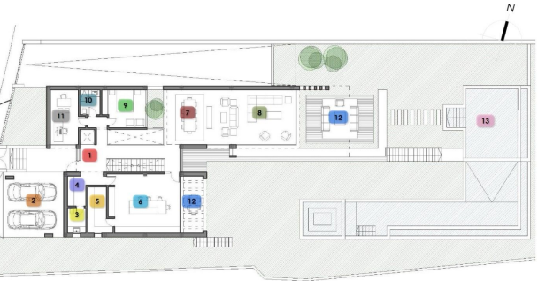
HOUSE SOUTH GROUND FLOOR
