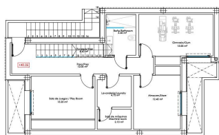
BASEMENT FLOOR (OPTIONAL)
