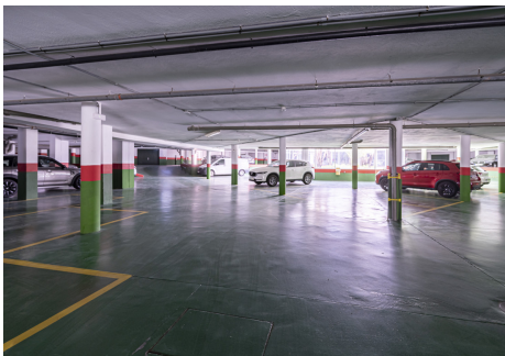
Virtual Decoration
